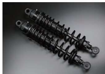
NITRON STEALTH TWIN R3 Series JPY ¥122,000 TST02SS Equips 1way damping adjusters / Internal reservoir tank model
